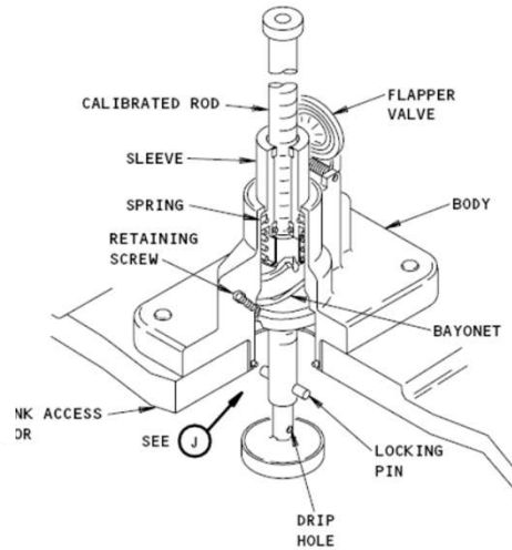
FUEL MEASURING STICK (EXAMPLE)
